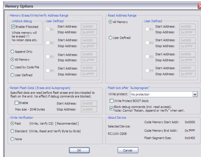
Figure 3: FlashPro-CC Memory options for block Debug interface
