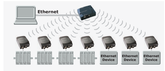
Bluetooth Ethernet Port Adapters (EPA) for connecting ethernet devices to an ethernet infrastructure via the Wireless Network Platform (WNP) in Access Point mode.
