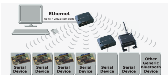
Wireless Network Platform (WNP) in Terminal Server mode. Serial devices are wirelessly connected to an ethernet infrastructure. The serial devices are accessed via virtual com-ports presented on the ethernet network.
